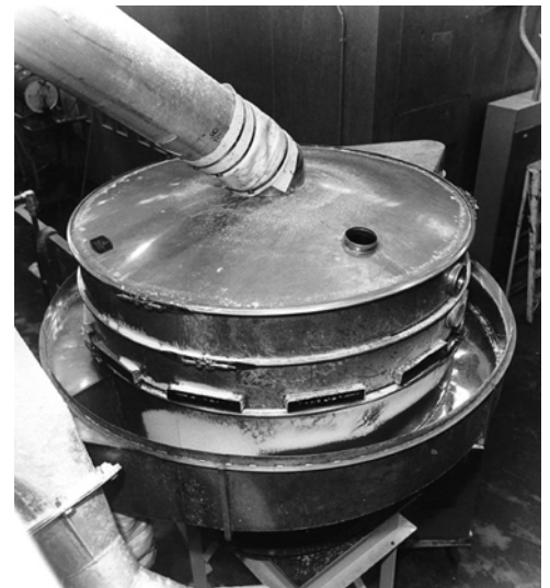
Clumps of oversize polyethylene pellets are fed into center entrance of the separator.
